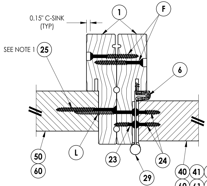
5 HORIZONTAL CROSS SECTION Outswing shown (Inswing similar)
