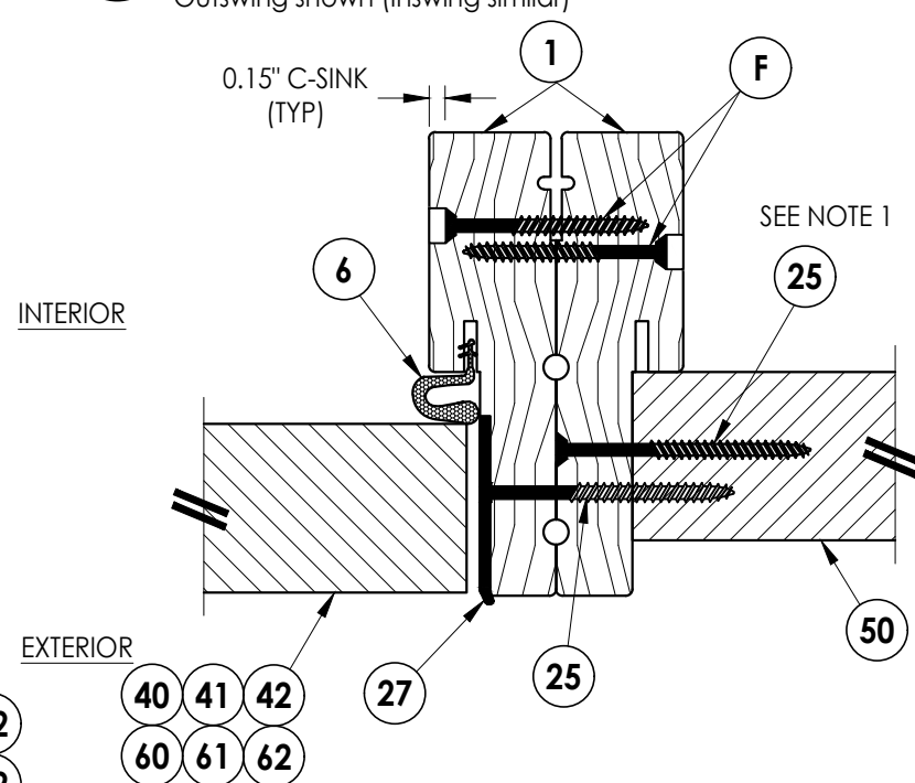
6 HORIZONTAL CROSS SECTION Outswing shown (Inswing similar)
