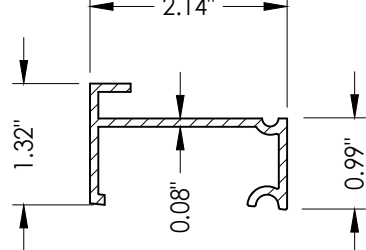
77 SIDELITE SPACER Inswing
